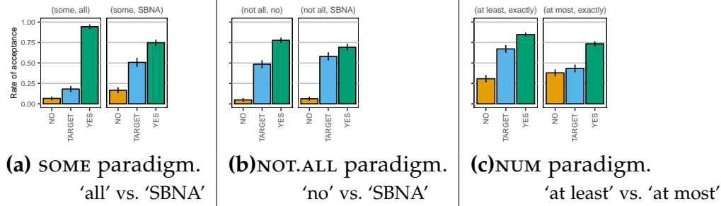
Figure 2: Proportion of ‘yes’ responses for each pair of QUANTIFIERS and each TYPE of item. NO cases made both rules attached to the quantifiers false; YES cases made them both true; and TARGET cases made one of them true and the other false. Error bars represent the standard error of the within-subject mean. Results are grouped by ‘paradigm’, i.e. pairs of QUANTIFIERS which meaningfully share one member (‘some’, ‘not all’, or ‘exactly n ’) and are used for the comparison between their other members.
