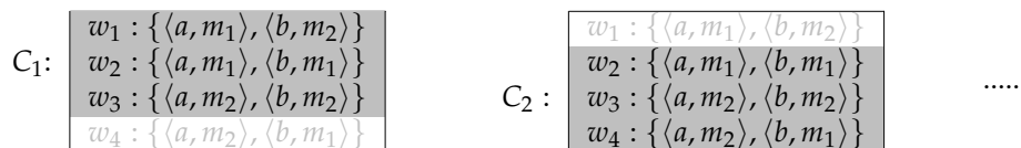
Figure 5: World grouping yielded by (108)
