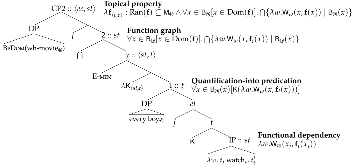
Figure 4: Composition of the \nabla -question which movie did every boy watch?
