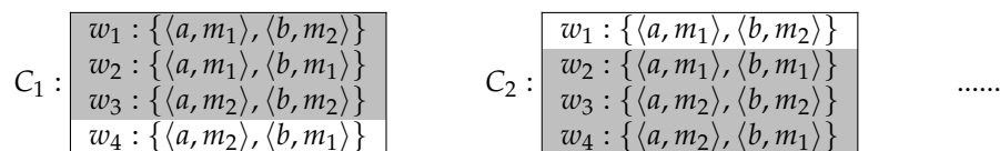
Figure 6: World grouping yielded by (87)
