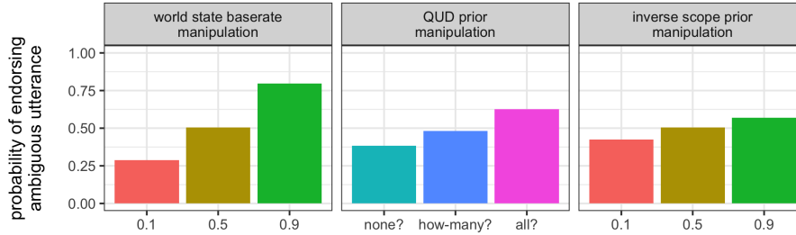
Figure 2: Model predictions for ambiguous utterance endorsement (e.g., Every horse didn't jump over the fence ) in a not-all scenario (e.g., one-out-of-two horses jump over the fence). Lower endorsement probability corresponds to less adult-like (i.e., more child-like) behavior. For the QUD factor, the favored parameter value receives most of the prior probability weight ( P(\textit{favored}) = 0.9 ). For the processing variable (scope), the prior corresponds to how strongly the inverse scope is favored.
