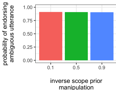
Figure 3: Model predictions for ambiguous utterance endorsement when total-success world states are favored ( b_{suc} = 0.9 ) and the optimal QUD is favored ( P(\mathbf{all?}) = 0.9 ).
