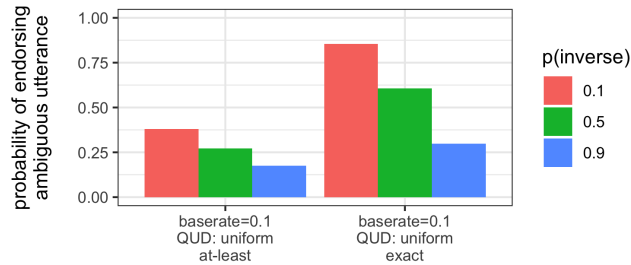
Figure 6: Model predictions for ambiguous two-not endorsement in a 2-OF-4 context with a low baserate of success is low (0.1) and QUD uncertainty (uniform QUD prior). On the left, we see predictions for an at-least semantics; on the right, we see predictions for an exact semantics.
