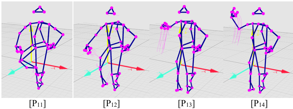
Figure 3: coreference condition
