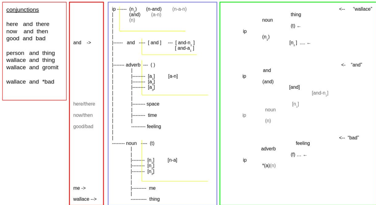
Figure 25 The “and” node is manually added as a child node of IP. The and node functions to predict the next (stm) symbol based on the previous (stm) symbol. This allows a false signal to occur on subsequent input of a dissimilar symbol: Wallace and *bad.
