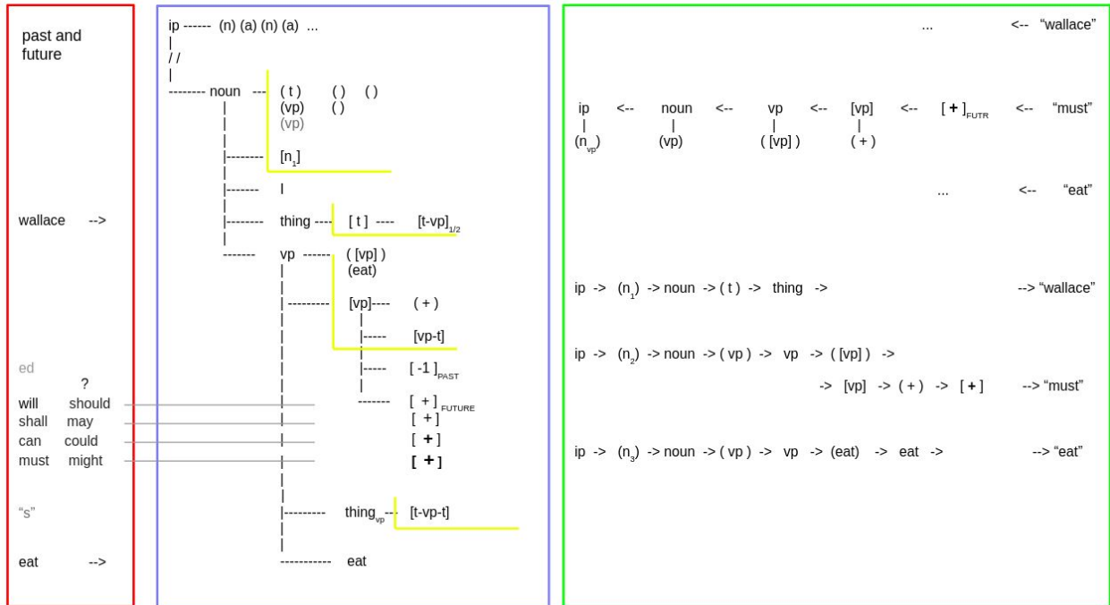
Figure 36 the future modal verbs bifurcate from the vp frame node using the stored value. The future modal (uncertain) verb forms can be alternatively externalized if ip.value = 0
