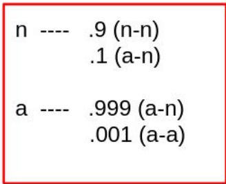
Figure: 18 the first level (fastest) prediction of the most probable next symbol using one level deep stored information
