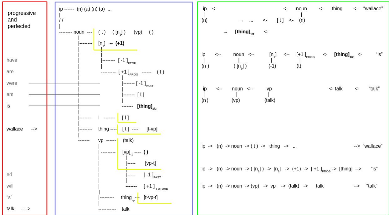
Figure 39 The [+1]_{\text{PROG}} node bifurcates on past, I and thing. The preactivation of the [\text{thing}]_{1/2} \rightarrow [+1]_{\text{PROG}} node allows an error check, ex: wallace *are talk ing. This implies that the information to generate the false * signal is stored in the [+1]_{\text{PROG}} node.
