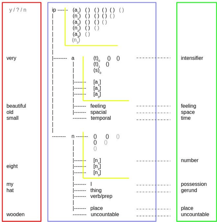
Figure 31 My eight beautiful very small old square English wooden hat boxes. The sequence of adjective archetypes corresponds to the ip subgraphs. Number, feeling, space, time, and noun.
