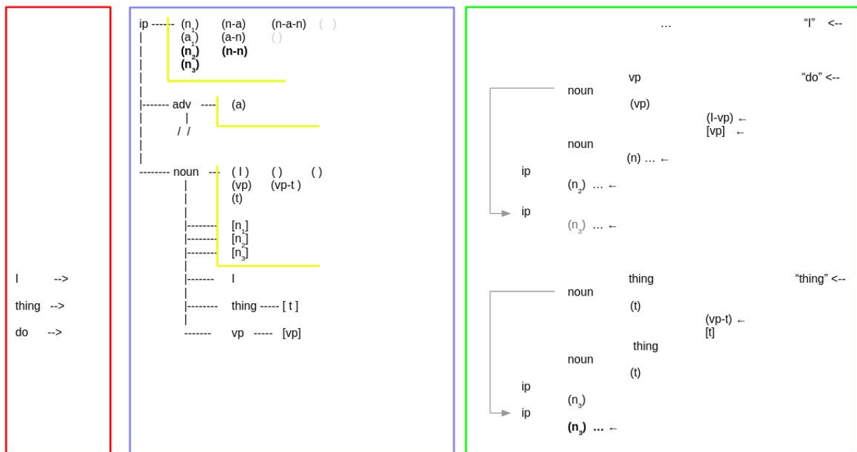
Figure 27 An [itm] sequence [vp] -> [vp-t] -> [t] causes an additional loop to execute in the noun branch, which allows the enhancement of internode connections in the IP (stm) memory, shown in bold.
