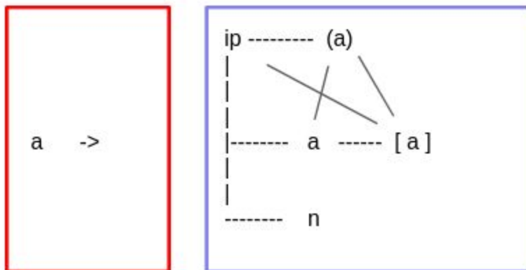
Figure 15 A long term memory node is formed by a reverse merge operation. The weights of the [ltm] nodes are initialized differently than the (stm) node and are then modified by a simple Hebbian mechanism that runs when the node fires. Weights are decreased when a node is touched, and increased if the touched node subsequently node fires.
