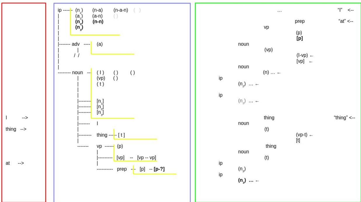
Figure 29 the preposition node
