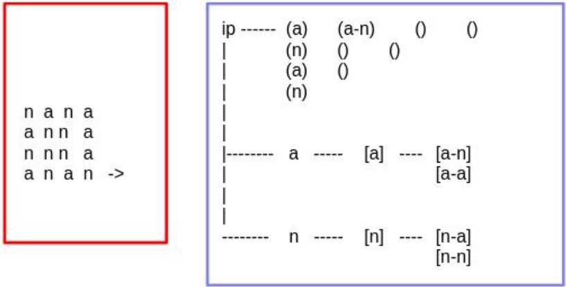
Figure 16 The first level [lrm] nodes, once formed, form sequential associations using the same mechanism as the (stm) nodes.
