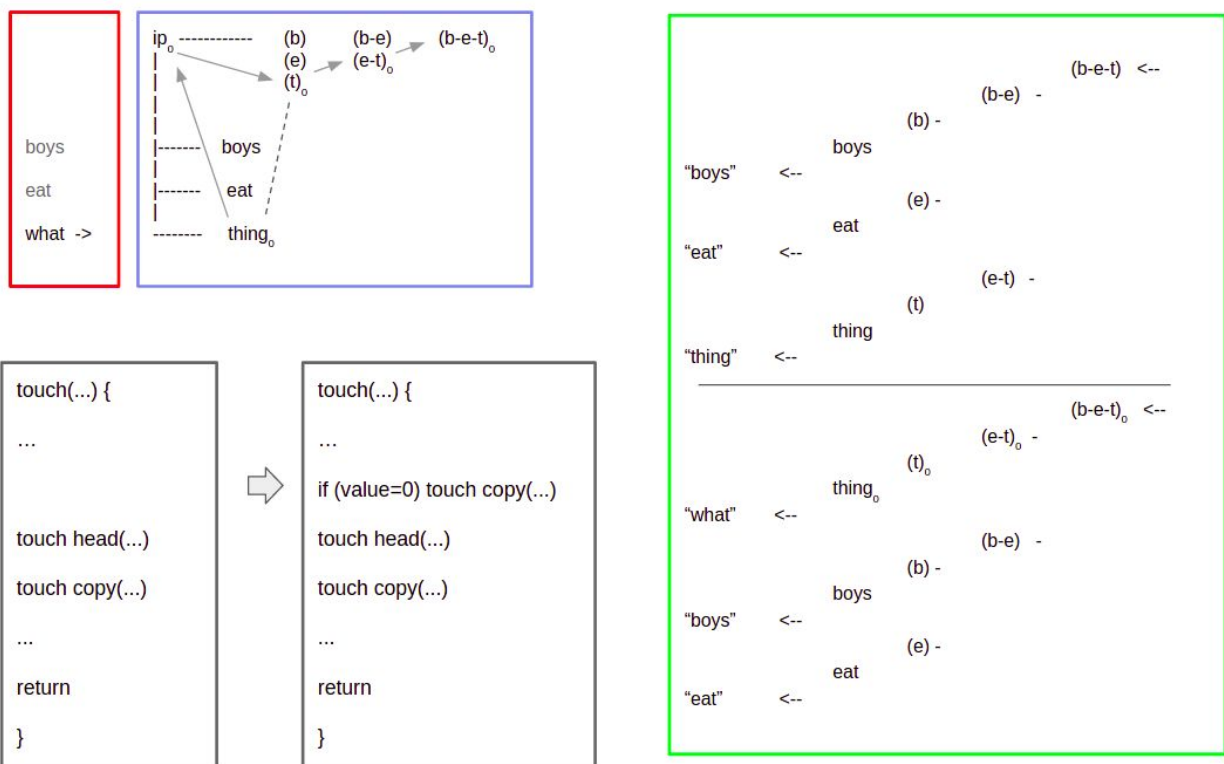
Figure 14 A mechanism for movement can be implemented using the stored values in the (stm) nodes. The input value is propagated to the (stm) nodes as shown, and the single line modification to the pseudocode will alter the output ordering from "boys eat what" to "what boys eat".
