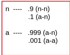
Figure 19 prediction of the next two symbols, with the lowest chance of being incorrect, using the first level branching probabilities predicted out to two symbols. The 'a' symbol is assumed optional and does not count as incorrect if not present.
