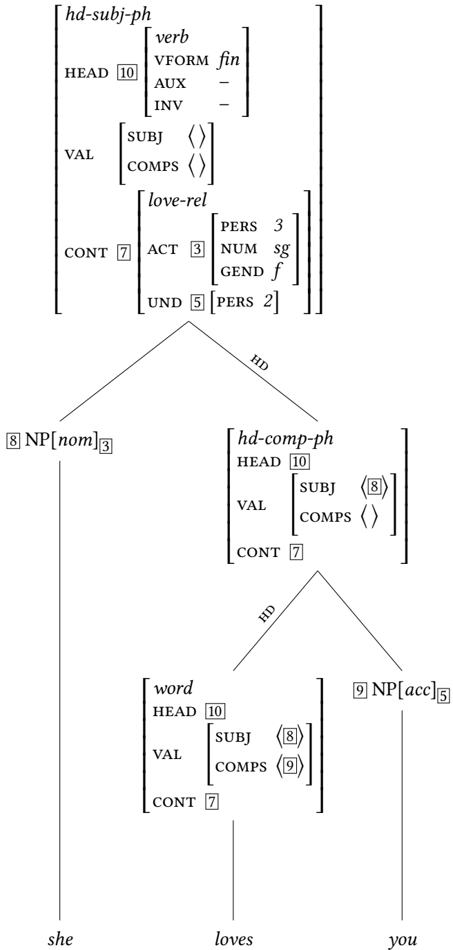
Figure 3: Shorthand HPSG representation of (1)
