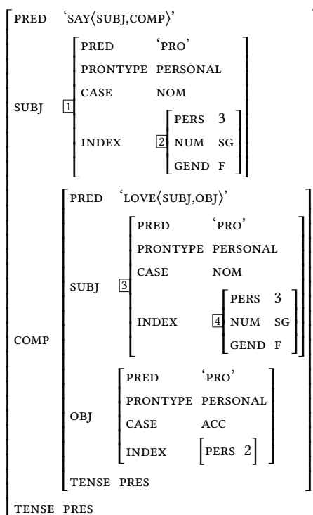
Figure 17: F-structure for (37)
