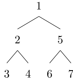
Figure 4: Depth-first search
