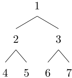
Figure 3: Breadth-first search
