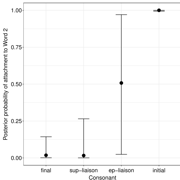
Fig. 2 Posterior probability of attachment to Word2 as a function of consonant type (mean and 95% CI)
