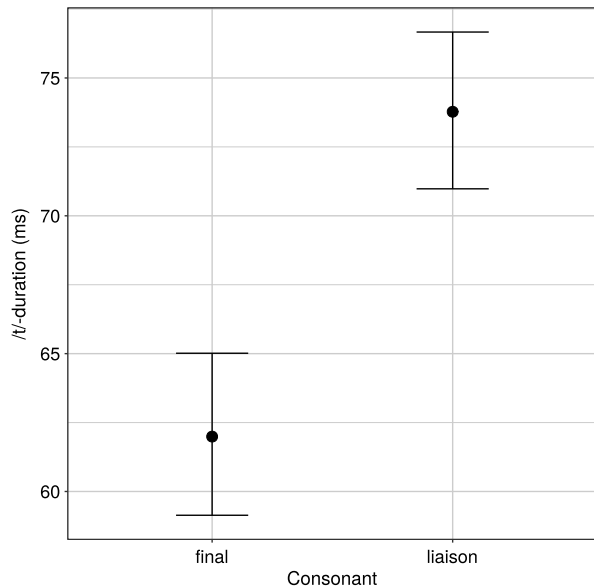
Fig. 5 Posterior distribution of consonant duration (ms) for stable word-final /t/ and liaison /t/ (mean and 95% CI)
