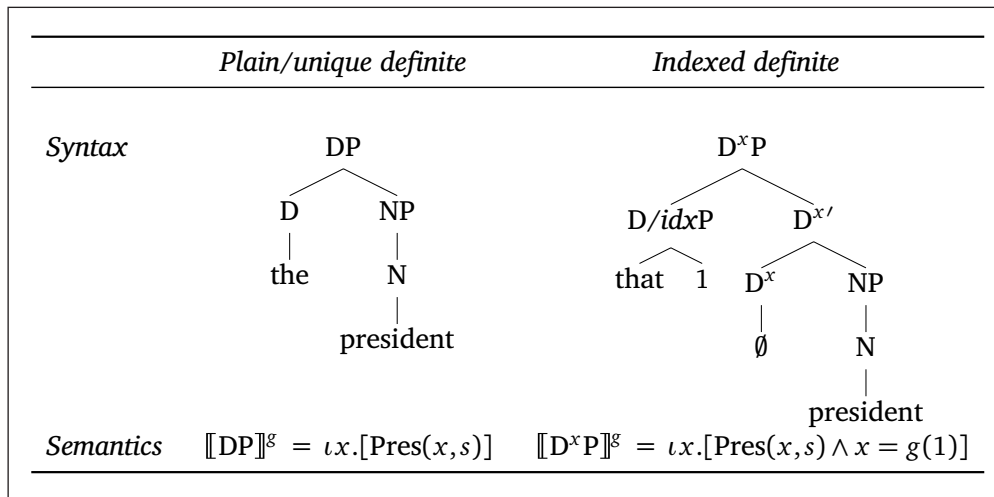
Figure 1: Plain versus indexed definiteness.
