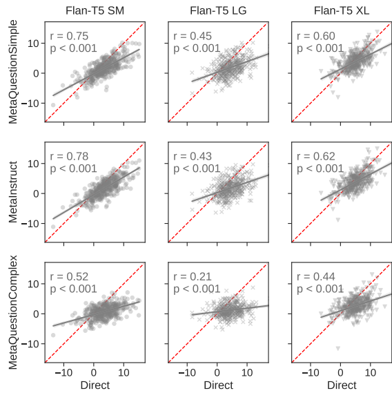
(a) Flan-T5
