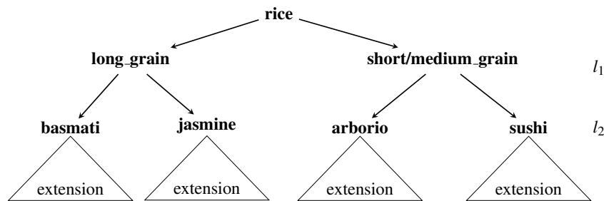
Figure 4: Subkinds at each level have Disjoint Extensions
