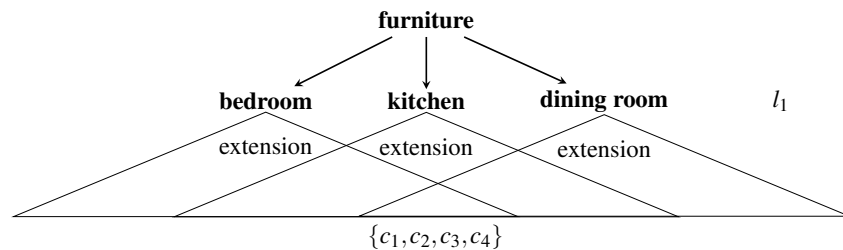
Figure 5: Subkinds at l_1 have Overlapping Extensions
