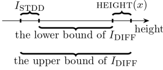
Fig. 1: The meaning of tall (see (24))
