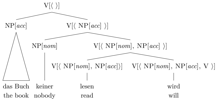
Figure 8: Formation of a verbal complex and scrambling of arguments (simplified version)
