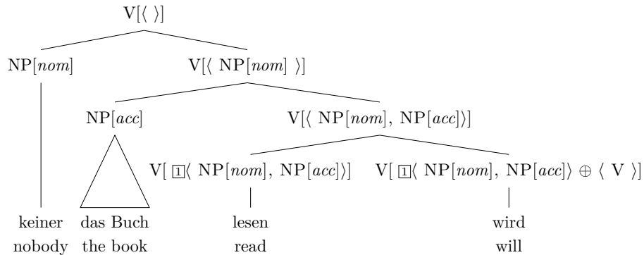
Figure 7: Formation of a verbal complex and realization of arguments in normal order (simplified version)
